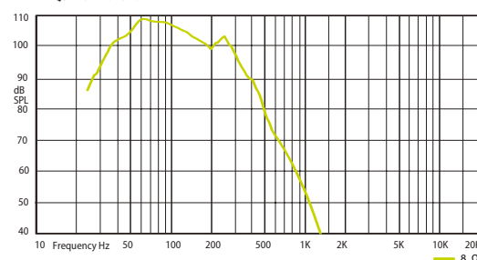
FREQUENCY RESPONSE
