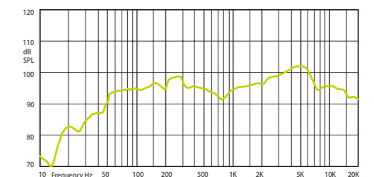
FREQUENCY RESPONSE
