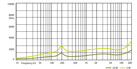
IMPEDANCE
