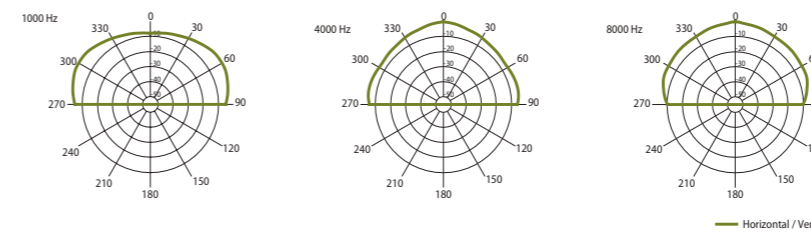
HORIZONTAL / VERTICAL POLAR DIAGRAMS
