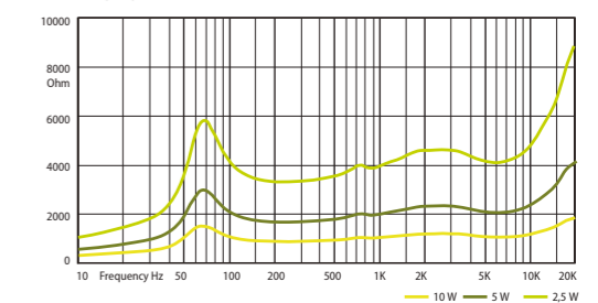
IMPEDANCE
