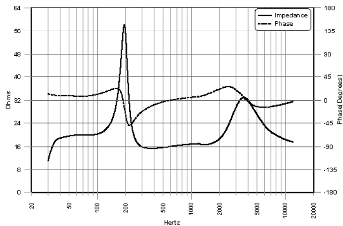
Phase/Impedance Response
