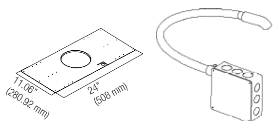
Pre-Construction Bracket (AC-CMEZ4-PCB)
