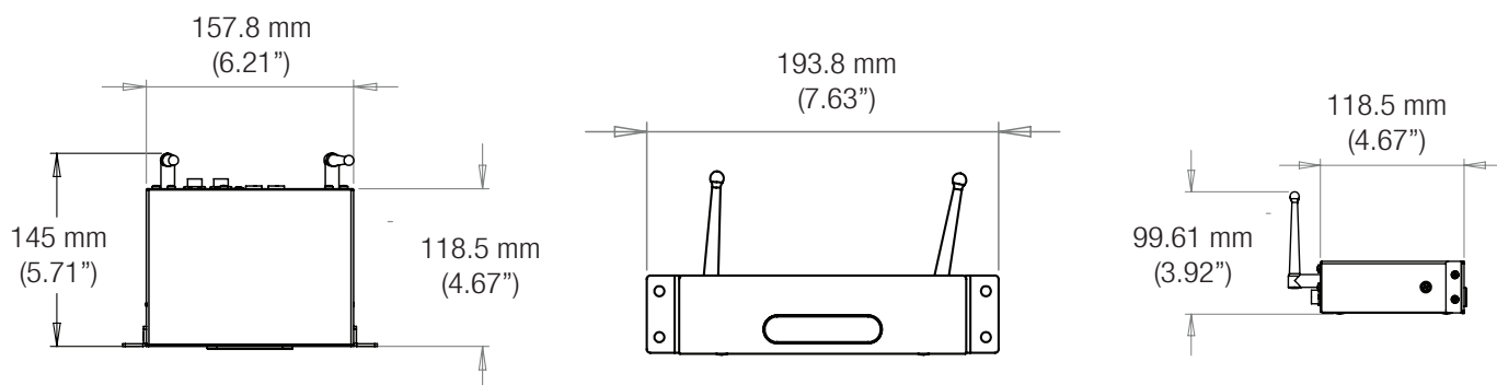
WLL-RX1p-II Receiver
